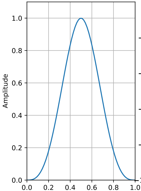
Bohman Window (64 points)
